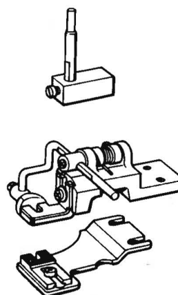
Shank Button Attachment 142570-101
