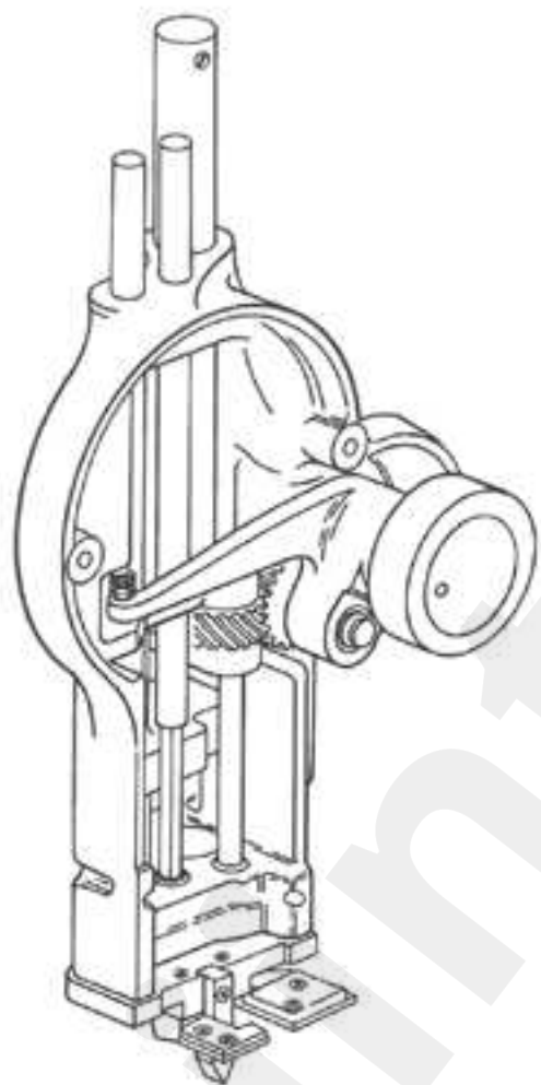
Figure 28. Sharpener Housing Assembly (Assembled, Rear View)
