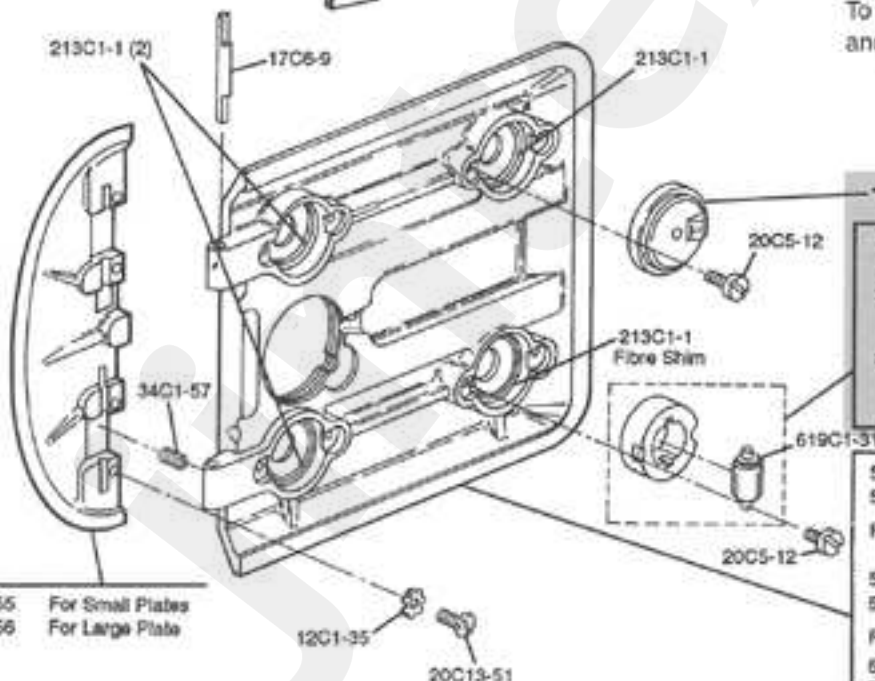
Figure 33. Standard and Baseplate Assembly (Exploded View)
