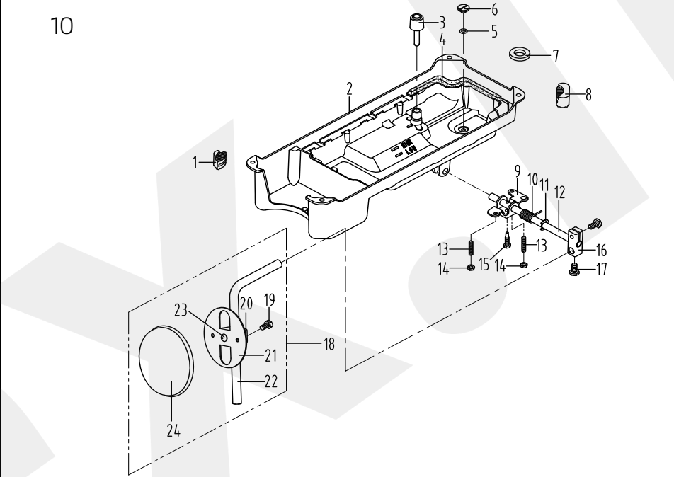
10. 油盘、膝抬压脚组件/Oil Ceservoir,Knee Lifter Components
