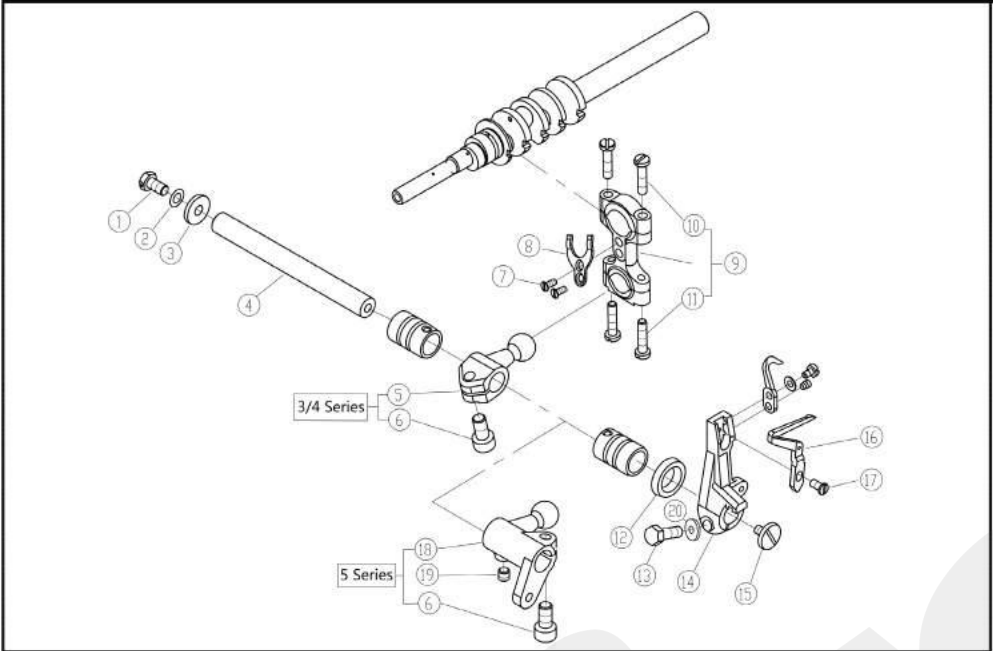
十三、下弯针部件/Lower Looper Drive Mechanism
