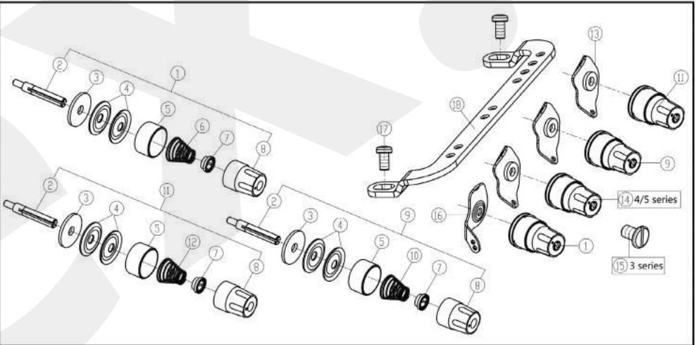
五、夹线部件/Thread Tension Mechanism
