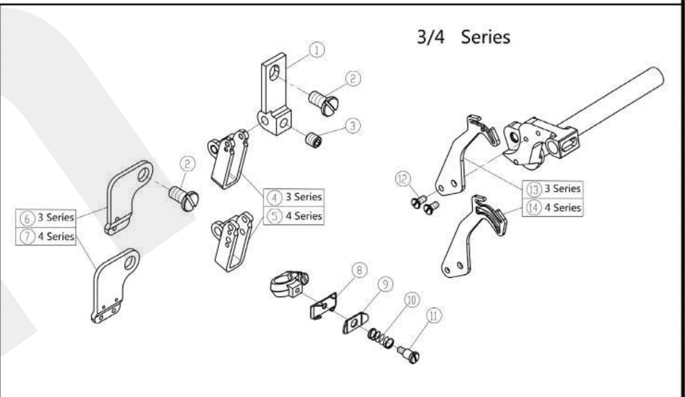
七、过线机构(2)/Thread Guide and Thread Takeup(2)
