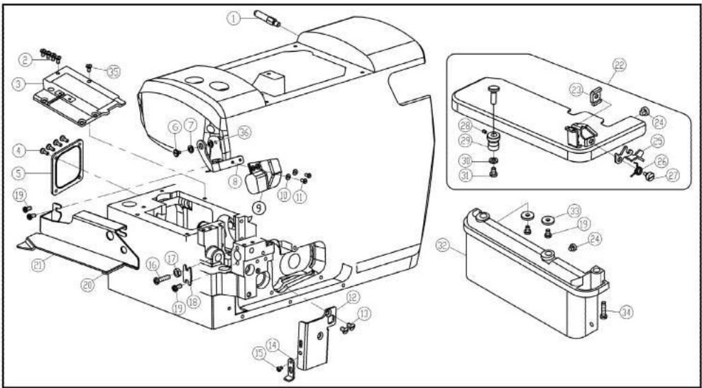
三、机壳机罩部件(2)/Cover (2)
