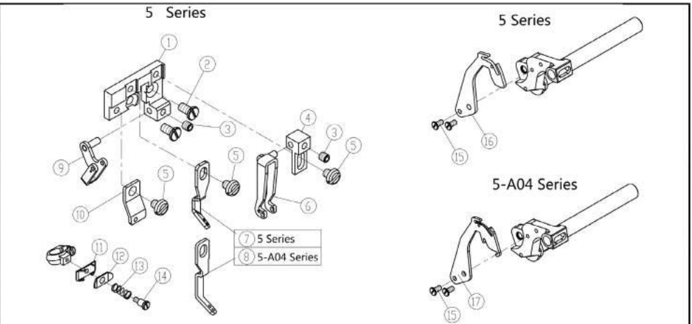
六、过线机构(1)/Thread Guide and Thread Takeup(1)
