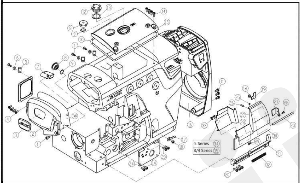
二、机壳机罩部件(1)/Cover (1)
