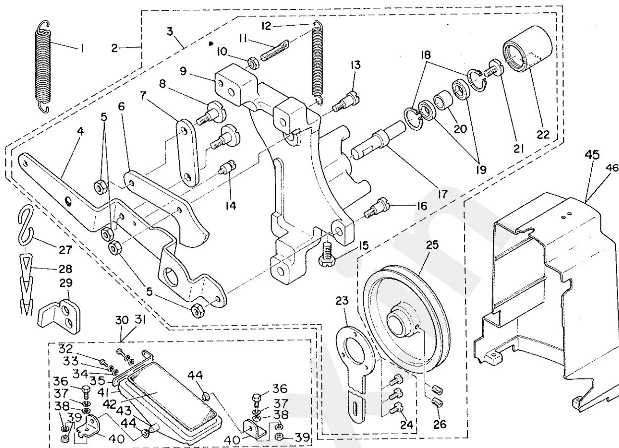
(14) LK-1850-P PEDAL TYPE CLAMP FOOT LIFTING DEVICE 足踏式押入上げ装置
