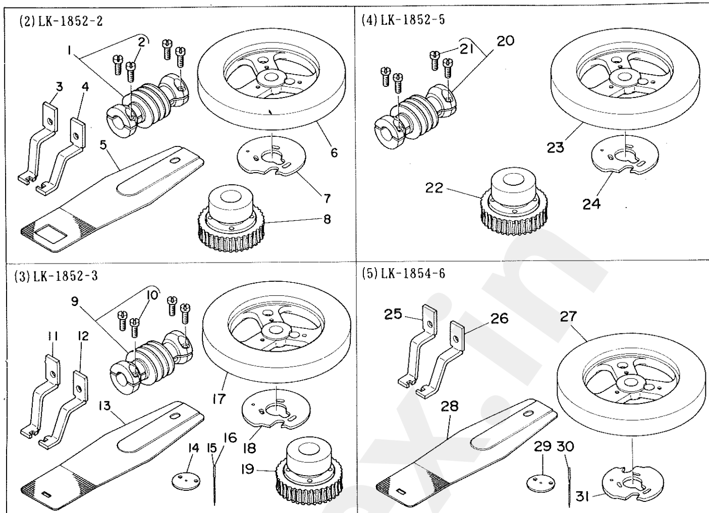
(2) LK-1852-2 SMALL BAR TACKING MACHINE (28 STITCHES) 28針小門止めマシン
