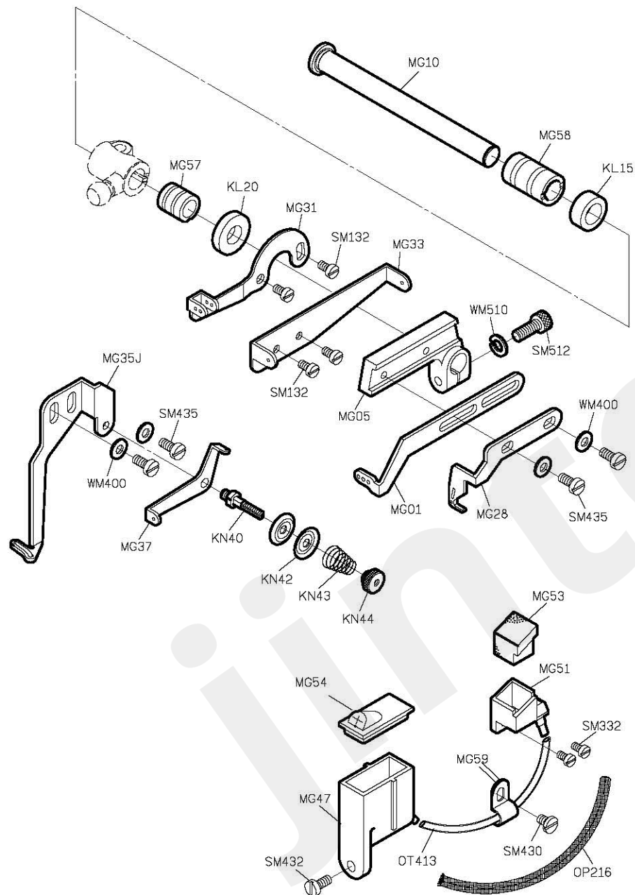
PARTS LIST FOR MG GROUP
