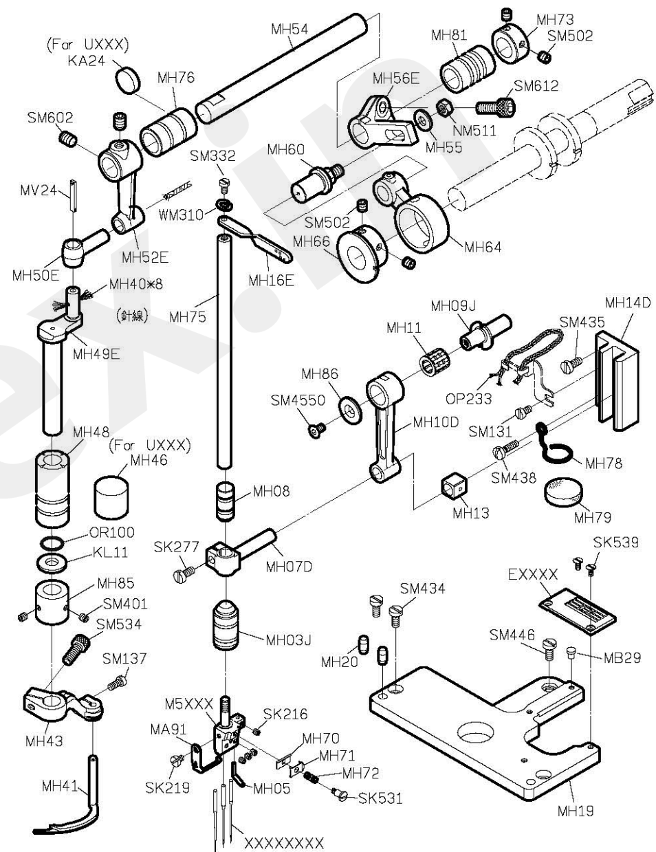
PARTS LIST FOR MH GROUP
