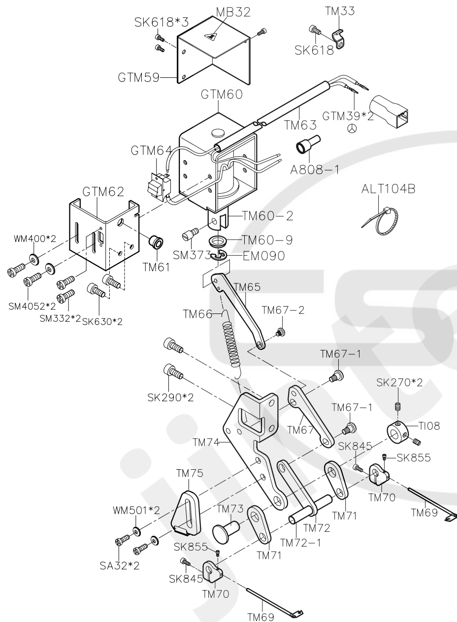
PARTS LIST FOR TM (5) GROUP
